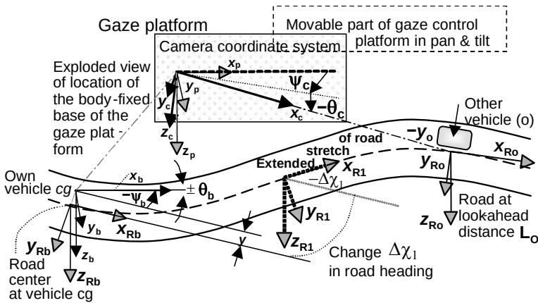
Figure 2.9. Coordinate systems for a general scene with own vehicle (index b) and one other vehicle (index o) on a curved road
