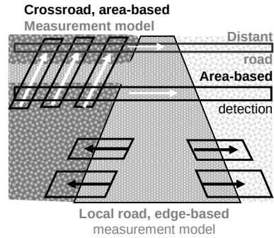
Figure 5.5. Crossroad detection in look-ahead region further away.
