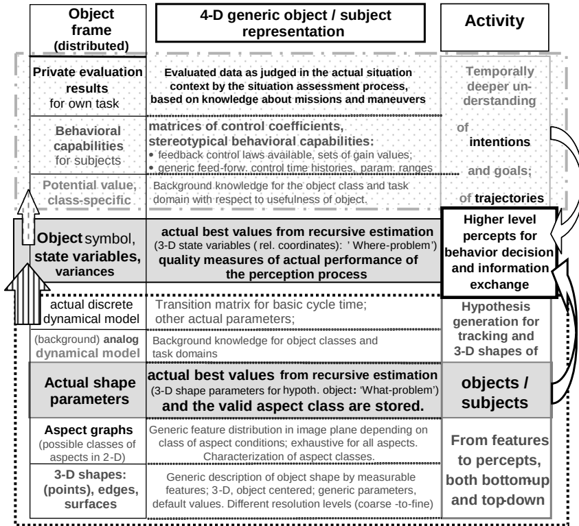
Figure 13.2. Summary of representational framework for objects/subjects in the 4-D approach to real-time vision (distributed realizations in the overall system, in general). Legend: black = actual values of dynamic object database (DOB); gray = background knowledge.
