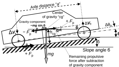
Figure 3.18. Longitudinal acceleration components going uphill: Forces, torques, and orientation changes in pitch
