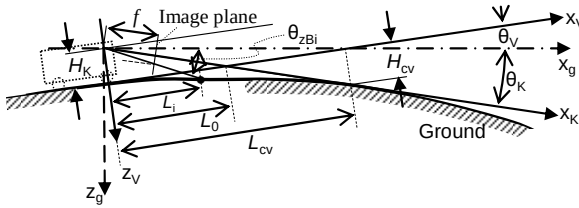
Figure 9.5. Negative vertical curvature analysis including cusp at L_{cv} with self-occlusion; magnitude of L_{cv} is ill defined due to the tangency condition of the mapping ray
