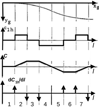
Figure 7.11. Clothoid road section: Top in Cartesian coordinates x, y ; second row: clothoid parameters C_{1h} = dC/dl ; third row: curvature C over arc length; fourth row: dC_{1h}/dl as Dirac impulses (step jumps in C_{1h} )
