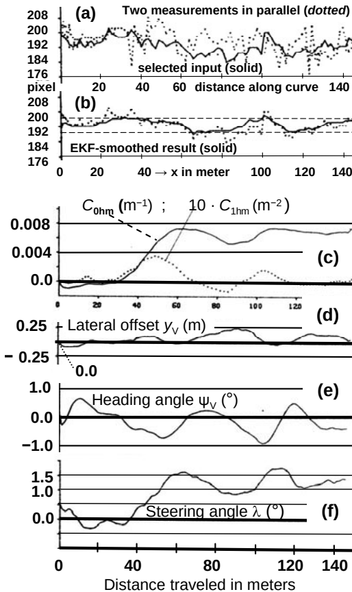
Figure 9.2. From noise corrupted measurements of edge feature positions ( dots , top graph (a)) via pre-selection through expectations from the process model [ dots in graph (b) = solid curve in (a)] to symbolic representations through high-level percepts: (c) road curvature at cg location of vehicle C_{0hm} and smoothed (averaged) derivative term C_{1hm} (multiplied by a factor of 10 for better visibility). (d) Lateral offset y_v of vehicle from lane center; lane = right half part of road surface (no lane markings except a tar-filled gap between plates of concrete forming the road surface). Note that errors were less than 25 cm. (e) Heading angle \psi_v of vehicle relative to road tangent direction ( |\psi_v| < 1^\circ ). The bottom graph (f) shows the control input generated in the closed-loop action-perception cycle: a turn to the right with a turn radius R of about 160 m ( = 1/C_{0hm} ) and a steering angle between \sim 1 and 1.7^\circ , starting at \sim 40 m distance traveled.
