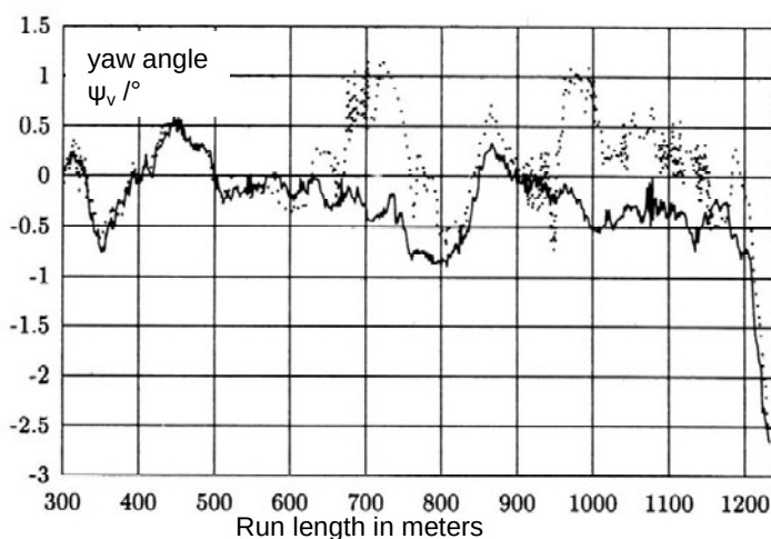
Figure 9.19. The effects of pitch motion modeled ( solid line ) or neglected ( dotted line for \theta = \text{constant} ) on other variables not directly involved in this degree of freedom; here: yaw angle estimation when quality of lane markings on each side differs (see text, after [Behringer 1996])
