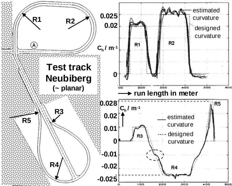
Figure 9.17. Test track for autonomous driving at UniBwM Neuberg, designed with different radii of curvature R_i , which are connected with and without clothoids (left: bird's-eye view). The right-hand part shows the design parameters (dotted) and the recovered curvatures from vision with test vehicle VaMoRs.
