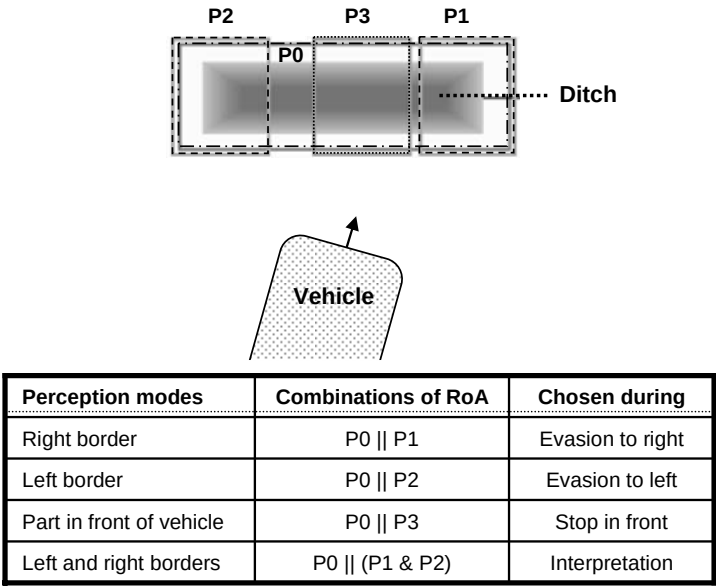
Figure 14.3. Regions of attention (RoA) for saccadic gaze control approaching a ditch of size larger than the field of view
