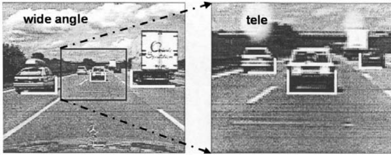
Figure 11.22. Five objects tracked in front hemisphere; in the own lane only the vehicle directly ahead can be seen (by both cameras). In neighboring lanes, the tele camera sees the second vehicle in front.
