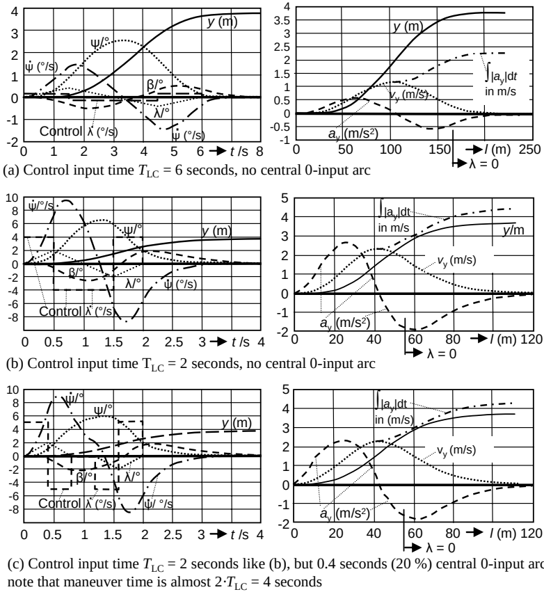
Figure 3.27. Comparison of lane change maneuvers with fifth-order dynamic model at a speed of V = 100 km/h (27.8 m/s) and realistic steer rate inputs. The amplitude A is adjusted such that the lateral offset y_f is exactly one lane width of 3.75 m after the transients have settled. Left column shows the variables (over time): d\lambda/dt = steer rate (—) in (°/s); angle \lambda (····) in (°); slip angle \beta (---) in (°); d\psi/dt = yaw rate (— · —) in (°/s), angle \psi (····). Right column the variables (over distance): lateral acceleration a_y (---) in (m/s²) and the integral of its magnitude over time (— · —); lateral velocity v_y (····); offset y (—); integral of magnitude of a_y (dash-dotted line).
