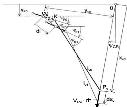
Figure 10.11. Gaze control in phase 3 for precisely determining angle \psi_{CR} and width b of the crossroad at an intersection.
