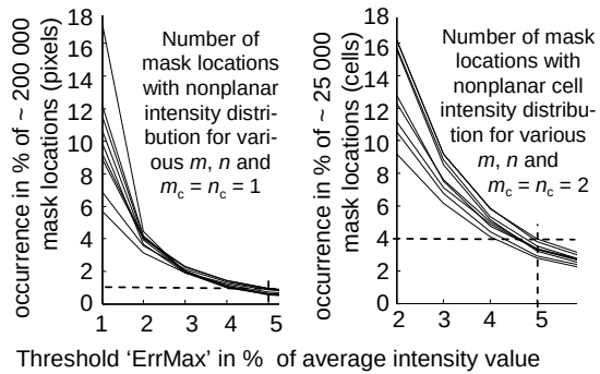
Figure 5.26. Relative number of nonplanar mask locations as a function of parameters for mask element formation m , n , m_c , n_c . Note that in the right part \text{ErrMax} starts at 2%; in the left part, which represents working on the pixel level, the relative frequency of nonplanar regions is down to \sim 4\% for this value.
