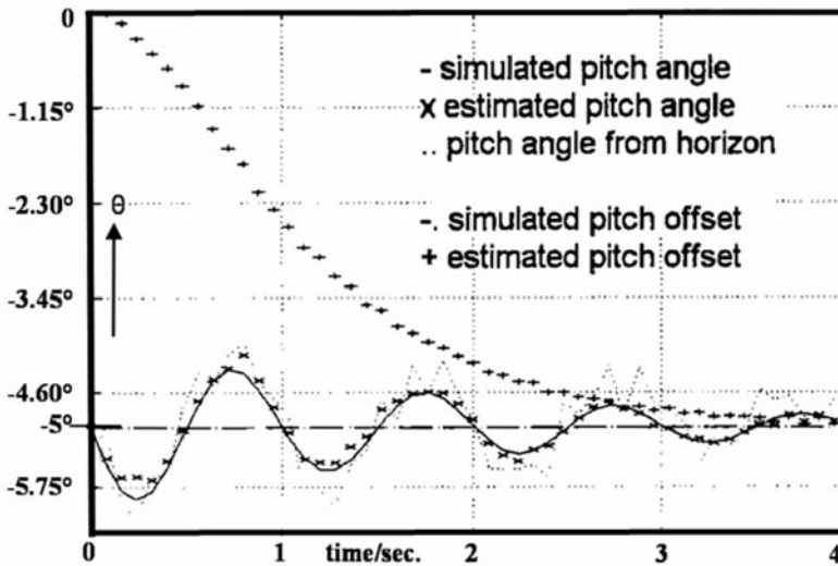
Figure 9.13. Estimation of pitch angle in simulation: Damped pitch oscillation (1 Hz, 1°) and offset (−5°). Convergence from \theta_{\text{offs}} = 0 occurred in \sim 4 s.
