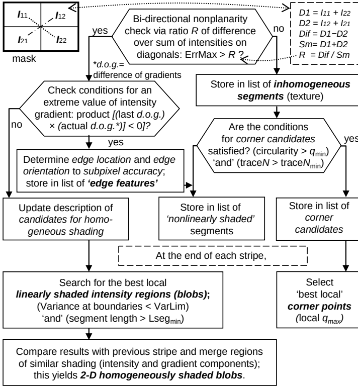
Figure 5.21. Decision tree for feature detection in the unified blob-edge-corner method (UBM) by local and global gradients in the mask region
