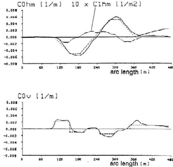
Figure 9.7. Simulation results comparing input model (dashed) with curvatures recovered from real-time vision (solid lines). Top: horizontal curvature parameters; bottom: Vertical curvature.
