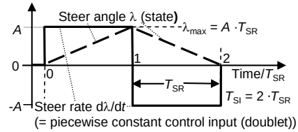
Figure 3.12. Doublet in constant steering rate U_{ff}(t) = d\lambda/dt as control time history over two periods T_{\text{SR}} with opposite sign \pm A yields a “pulse” in steer angle for heading change
