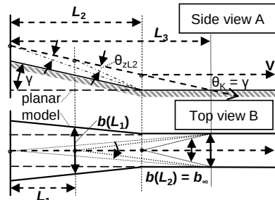
Figure 9.12. Two specific interpretations of the image in Figure 9.11: Hypothesis A: Constant lane width b_\infty and jump in slope angle \gamma at L_2 = L_{ch} (top right). Hypothesis B: Flat ground and linearly decreasing road width for l < L_2 : Parameter b_1 = (b(L_2) - b(L_1))/(L_2 - L_1) [dashed road boundary bottom right]
