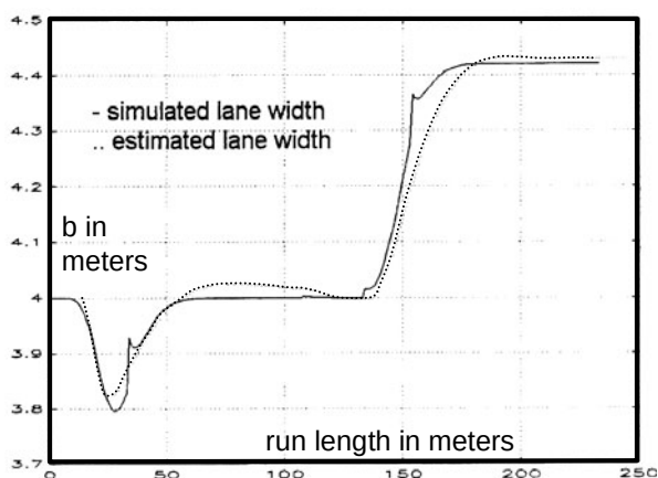
Figure 9.15. Simulation test for road width estimation: Imperfect software for lane width simulation generated small peaks and jumps ( solid curve ), which have not been removed on purpose to see the response of the estimation process ( dotted curve ). Nice smoothing and some overshoot occurred.
