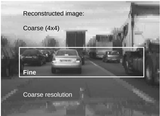
Figure 11.12. Highway scene similar to Figure 11.11 with more vehicles analyzed with UBM method in horizontal stripes; the outer regions are treated with coarse resolution (11.44R), while the central region (within the white box) covering a larger look-ahead range above the road, is analyzed on a fine scale (11.11R) (reconstructed images, see text)
