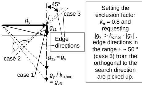
Figure 5.29. Limiting edge directions to be found in row-search around the vertical can be achieved by introducing limits for the ratio of gradient components ( |g_y| / |g_z| > k_{a,\text{hor}} ); (analogous for column search: k_{a,\text{hor}} need not be equal to k_{a,\text{vert}} )
