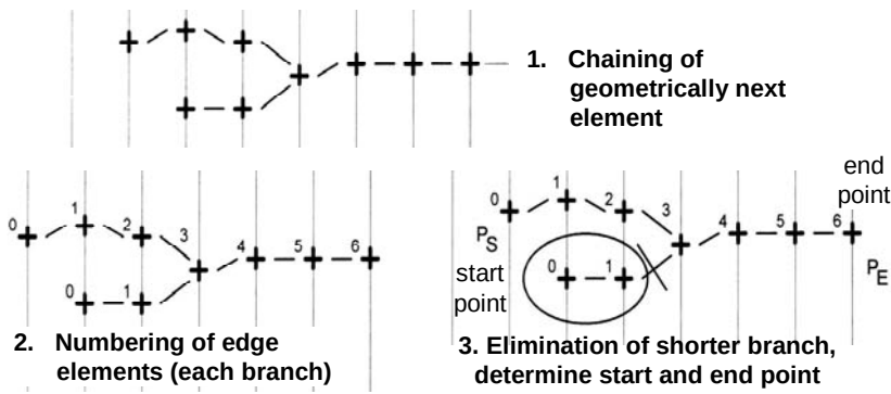
Figure 11.8. Contour generation from edge elements observing gestalt ideas of nearness and colinearity; below an upper limit for total contour length, only the longer one is kept
