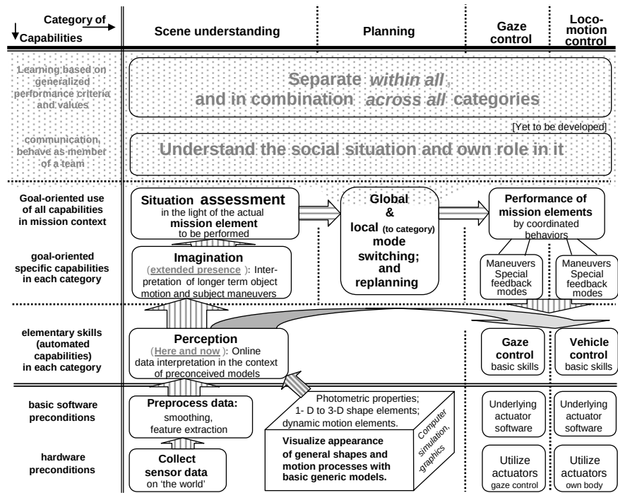
Figure 15.3. Differentiation of capability levels (vertical at left side) and categories of capabilities (horizontal at top): Planning happens at the higher levels only in internal representations. In all other categories, both hardware available (lowest level) and ways of using it by the individual play an important role. The uppermost levels of social interaction and learning need more attention in the future.
