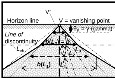
Figure 9.12. Two specific interpretations of the image in Figure 9.11: Hypothesis A: Constant lane width b_\infty and jump in slope angle \gamma at L_2 = L_{ch} (top right). Hypothesis B: Flat ground and linearly decreasing road width for l < L_2 : Parameter b_1 = (b(L_2) - b(L_1))/(L_2 - L_1) [dashed road boundary bottom right]
