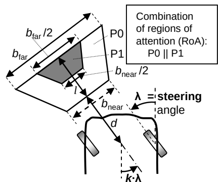
Figure 14.2. Linking gaze direction to steering angle for maneuvering
