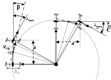
Figure 10.7. Theoretical limit for tightest turn possible: (1) Turn steering angle to maximum at standstill; (2) Drive circular arc until the direction of the crossroad is reached (here 90°); stop again. (3) Turn steering angle back to zero and start road running. Note that changing the steering angle \lambda at slow speed immediately turns the velocity vector; therefore, the circular arc driven starts at \beta and has to be driven till (90 + \beta)^\circ
