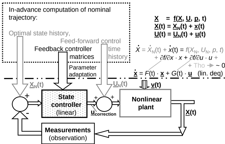
Figure 3.7. Approximation of a nonlinear process by superposition of a nominal nonlinear part and a superimposed linear part with a vector of perturbations \mathbf{v}(t)
